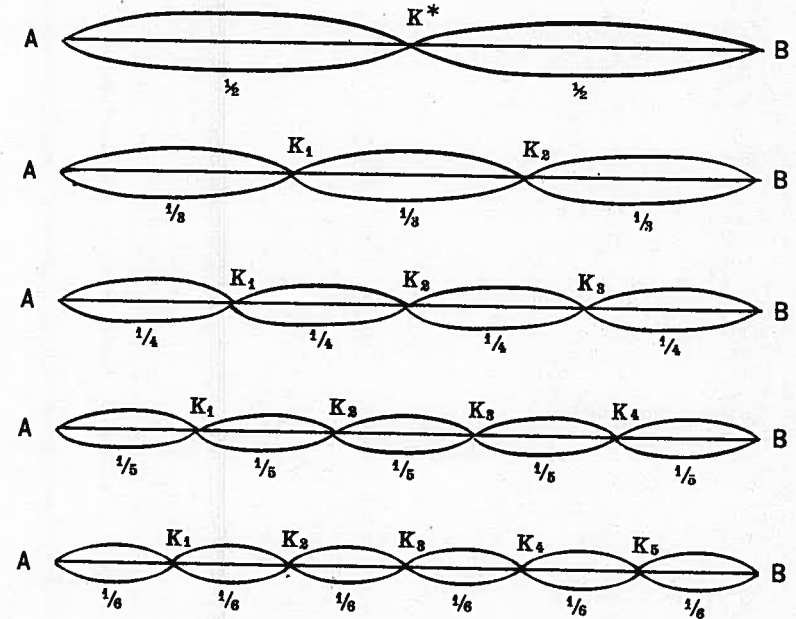
Figure 16. String nodes.
