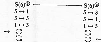
Figure 74. Transformation of S(6)Ⓞ → S(6)Ⓞ.
